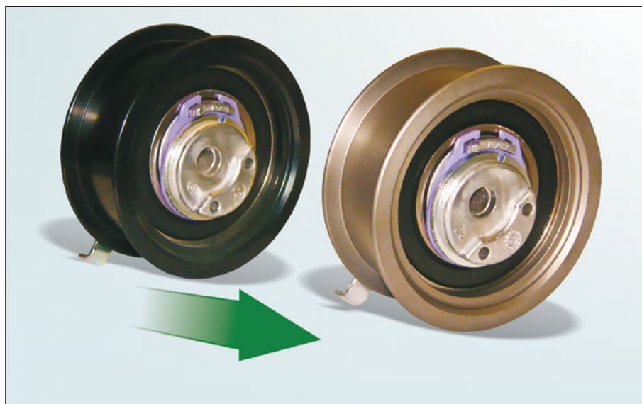
Image 1: Improved race coating — item no. 531 0524 30 shown here as an example
